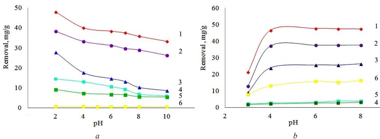
Fig. 4. Removal rate of: a – Cr(VI) and b – Co(II) as a function of pH (1 – HDTMA-Mont/nZVI, 2 – Mont/nZVI, 3 – nZVI, 4 – iron powder, 5 – HDTMA-Mont, 6 – Mont)
