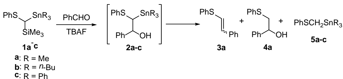
Scheme 1. Reactivity of stannyl-silanes 1a-c with benzaldehyde
