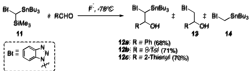
Scheme 3. Functionalization of benzotriazolyl-stannyl-silane 11 with aldehydes. Yields refer to isolated products. 5-10% of destannylated alcohols 13a-c was detected.
