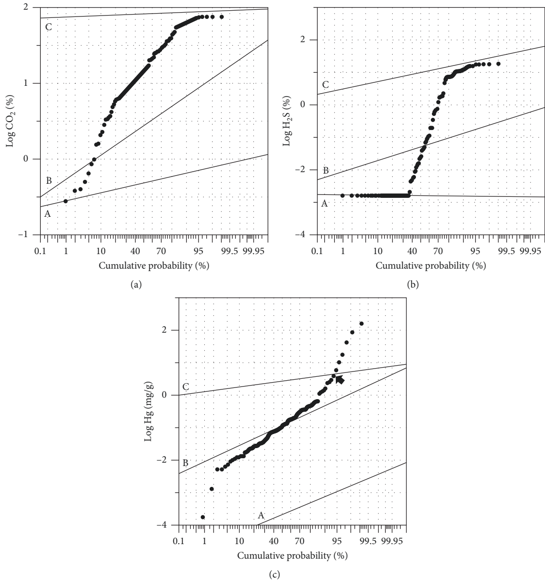
FIGURE 7: Probability plots of total \text{CO}_2 (a) and \text{H}_2\text{S} (b) concentrations in the soil gas and Hg (c) concentrations in the soils of the Lakki Plain.
