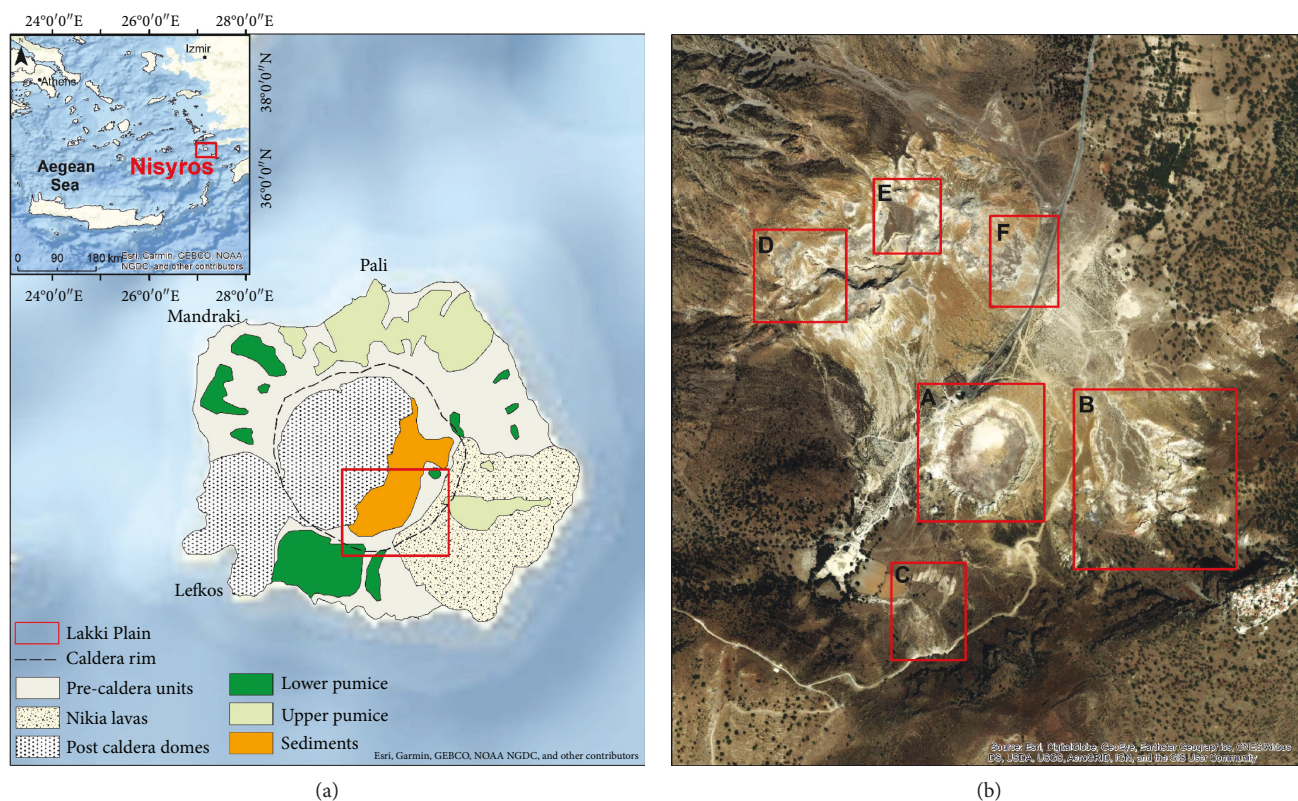
FIGURE 1: Simplified geologic map of the island of Nisyros (a) and sampling areas within the Lakki Plain (b). A = Stefanos crater; B = Kaminakia crater; C = Ramos fumaroles; D = Phlegeton crater; E = Mikros Polybotes; F = Lofos dome.
