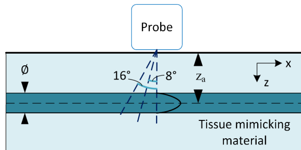
Fig. 2. Schematic of the experimental and simulations set-up.
