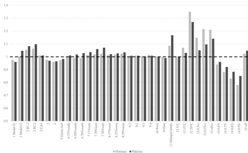
Figure 10. Results of the sensitivity analysis for the cities of Florence and Palermo. The values are normalized with respect to model 11.
