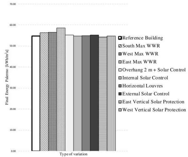
Figure 7. Final energy consumption for Palermo with respect to WWR and horizontal and vertical solar shadings
