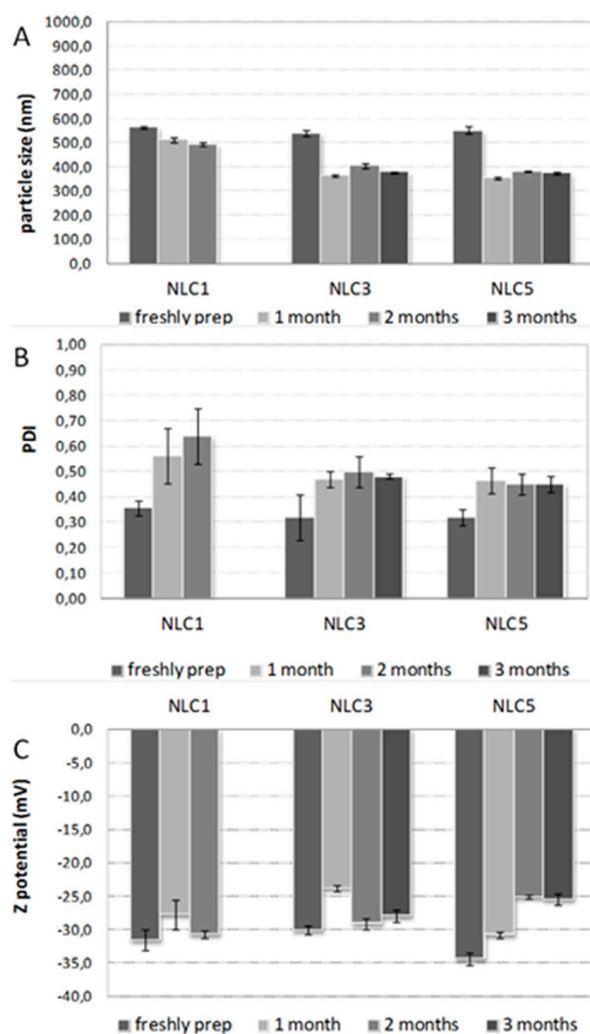
Figure 5. Stability studies of Tween ® 80-based NLC containing the drug as such (NLC1) or as P.M. (NLC3) or GR system with HP \beta CD (NLC5), freshly prepared and after 1, 2 and 3 months storage at 4 °C in terms of mean size (A), polydispersity index, PDI (B) and Zeta potential (C).
