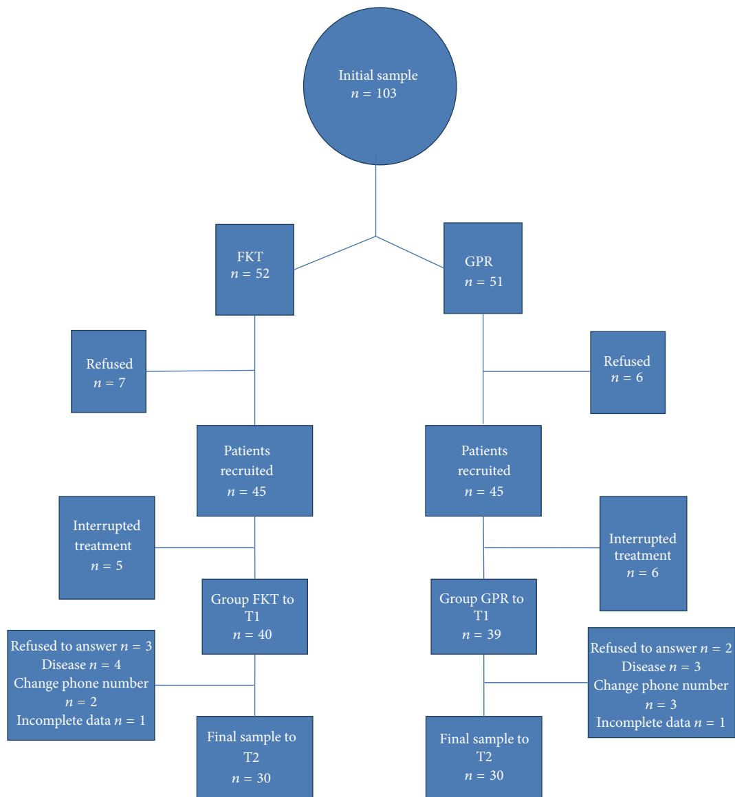
FIGURE 1: Study flowchart.
