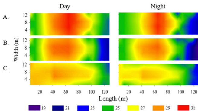
Figure 2. Maps of air temperature ( ^{\circ}\text{C} ) distribution across the poultry house in the day- and nighttime periods. Mean temperature in the first week (A), mean temperature in the second week (B) and mean temperature in the third week (C)
