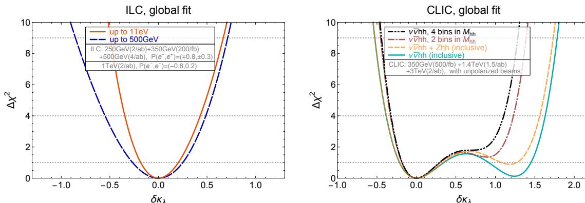
Figure 10. \Delta\chi^2 as a function of \delta\kappa_\lambda for the high-energy ILC (left) and CLIC (right) benchmarks. The results are obtained through a global analysis, profiling over all other EFT parameters.
