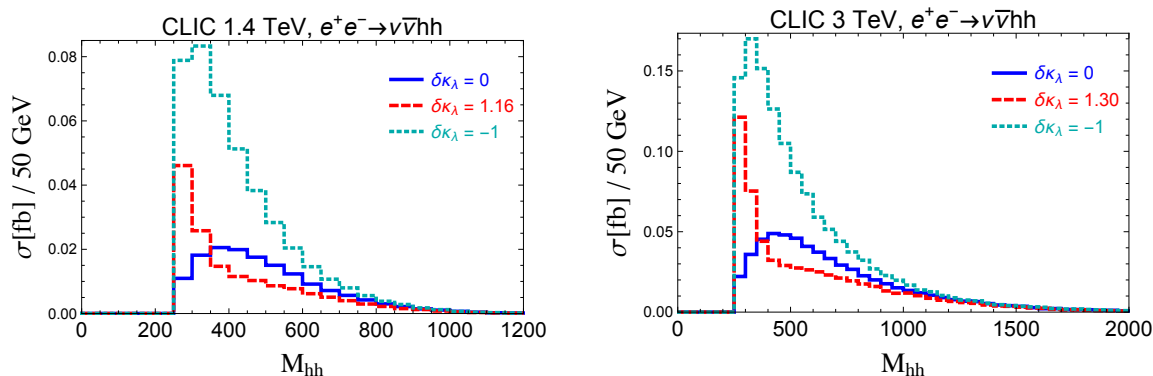
Figure 9. Invariant mass distribution of the Higgs pair in e^+e^- \rightarrow \nu\bar{\nu}hh at 1.4 TeV (left) and 3 TeV (right). The solid blue curves are obtained in the SM ( \delta\kappa_\lambda = 0 ). The red dashed curves are obtained with the other value of \delta\kappa_\lambda which leads to a cross section equal to the SM one. The cyan dotted curves are obtained for vanishing Higgs self-coupling ( \delta\kappa_\lambda = -1 ).
