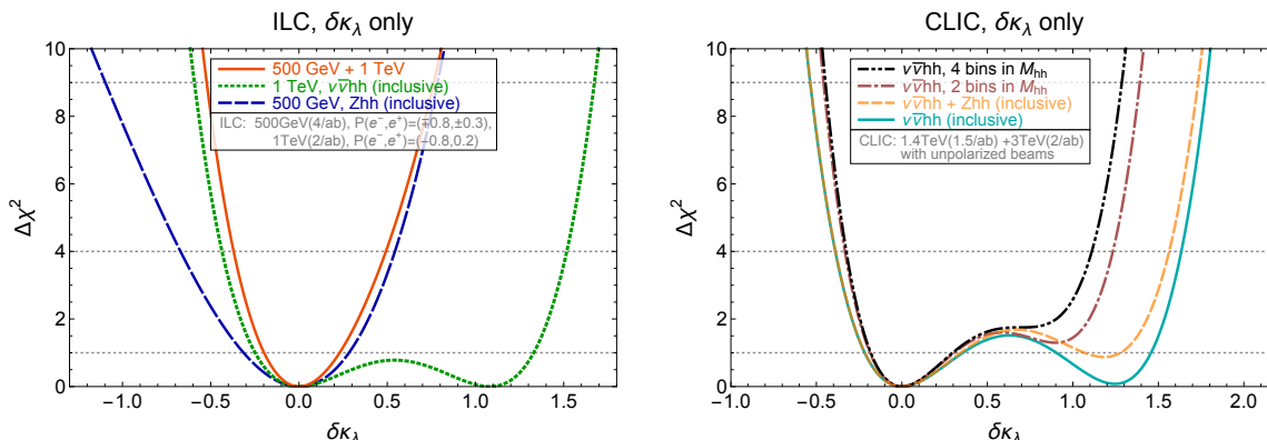
Figure 8. Chi-square for the exclusive fit of \delta\kappa_\lambda for various combinations of Higgs pair production measurements at the ILC (left) and CLIC (right).
