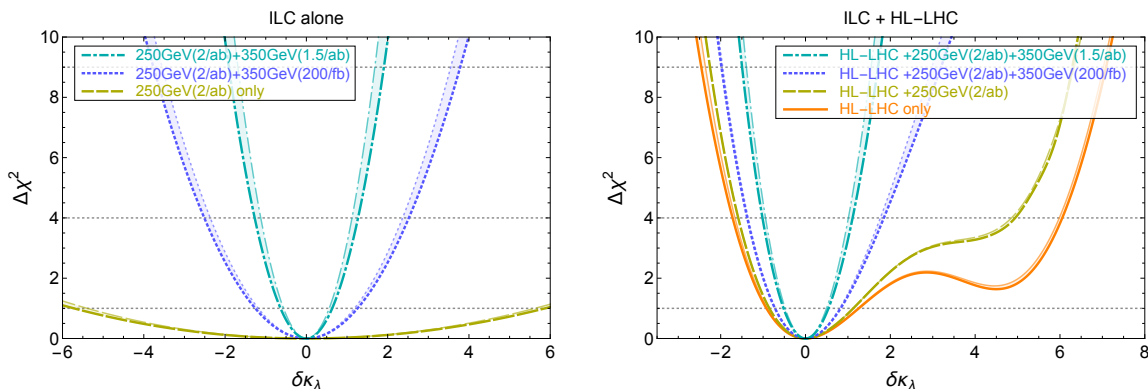
Figure 14. \Delta\chi^2 profiled over all EFT parameters but \delta\kappa_\lambda . Three run scenarios are considered for ILC, with 2\text{ ab}^{-1} at 250 GeV and \{0, 200\text{ fb}^{-1}, 1.5\text{ ab}^{-1}\} at 350 GeV, with luminosities equally split into P(e^-, e^+) = (\mp 0.8, \pm 0.3) beam polarizations. The shaded areas cover different assumptions about the precision of TGC measurements. Left: ILC measurements only. Right: combination with differential single- and double-Higgs measurements at the HL-LHC.
