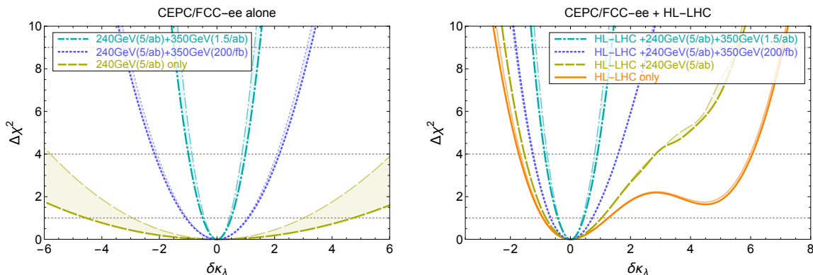
Figure 3. Chi-square as a function of \delta\kappa_\lambda after profiling over all other EFT parameters. Three run scenario are considered for circular colliders, with 5 \text{ ab}^{-1} at 240 GeV and \{0, 200 \text{ fb}^{-1}, 1.5 \text{ ab}^{-1}\} at 350 GeV, without beam polarization. The shaded areas cover different assumptions about the precision of TGC measurements. Left: circular lepton collider measurements only. Right: combination with differential single- and double-Higgs measurements at the HL-LHC.
