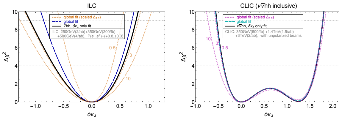
Figure 11. Left: Chi-square profiled over all EFT parameters but \delta\kappa_\lambda for ILC (up to 500 GeV). Right: the same for CLIC (no binning in M_{hh} ). Three scenarios are shown. The solid black curves correspond to the \delta\kappa_\lambda only fit from the double-Higgs measurements. The dashed blue/cyan curves correspond to the global fits in figure 10. The additional dashed curves are obtained by rescaling the uncertainties of single Higgs measurements (including e^+e^- \rightarrow WW ) by an overall factor. For example, \Delta_{1h} \times 10 denotes that the uncertainties of the single Higgs and diboson measurements are multiplied (worsened) by a factor 10.
