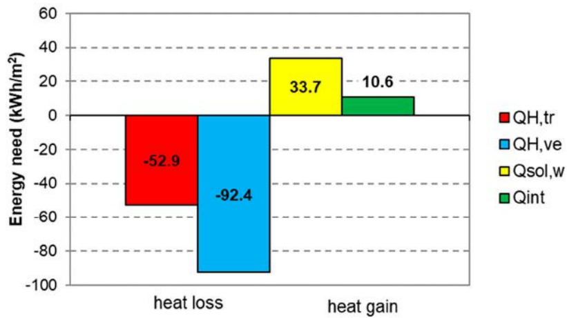
Figure 24. Energy analysis for the heating mode (in kWh/m 2 ).
