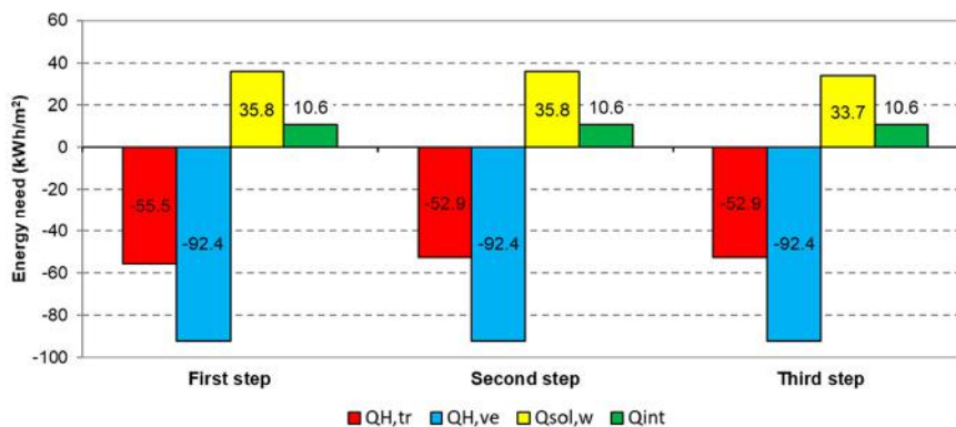
Figure 26. Comparison between energy analysis of the three different steps for the heating mode (in kWh/m 2 ).
