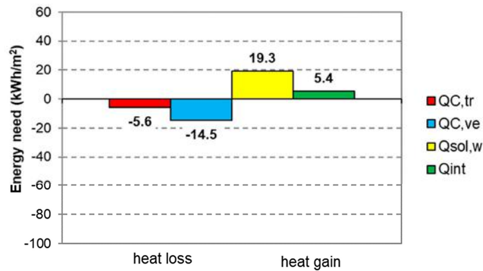
Figure 25. Energy analysis for the cooling mode (in kWh/m 2 ).
