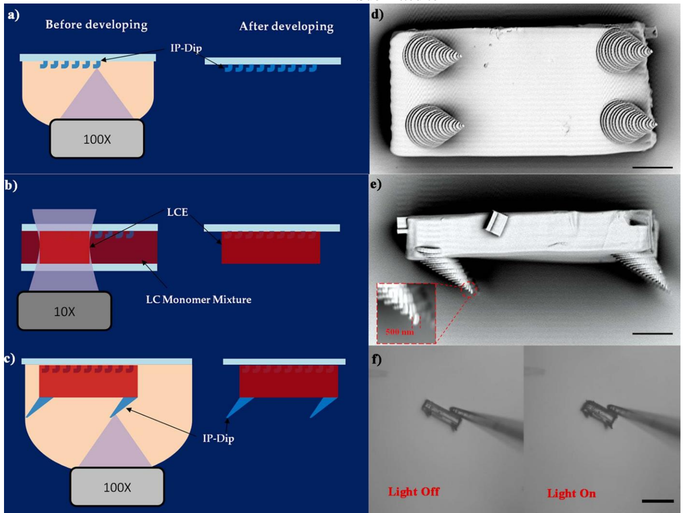
Figure 2. Fabrication of the microscopic walker. a) IP-Dip anchors were first fabricated on a rubbed polyimide coated glass by direct laser writing, followed by the developing process. b) A 10 \mu\text{m} gap cell was made by putting another PVA coated glass with parallel rubbing and infiltrated with the LC monomer mixture. The LCE body was made by the same laser writing system with a 10 \times microscope objective. c) Another drop of IP-Dip was applied, covering the fabricated structure and four conical legs were fabricated on the LCE body. d) SEM image of a micro-walker lying upside down. Scale bar is 10 \mu\text{m} . e) Side view of the micro-walker (scale bar: 10 \mu\text{m} ), with 500 nm leg tip shown in the inset. f) Actuation of the micro-walker under a 532 nm laser beam excitation (Scale bar: 50 \mu\text{m} ).
