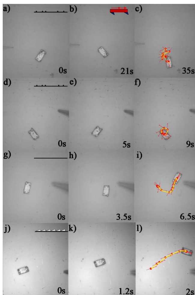
Figure 3. Surface dependent locomotion behaviors. Under the same chopped laser excitation (532 nm, 50 Hz, 10 W/mm 2 ), the 60 μm size microscopic walker: a)-c) , randomly walks on the PI coated glass surface; d)-f) , rotates with one leg stuck onto the PI coated surface; g)-i) , walks with self reorientation on the clean glass surface; j)-l) , walks in the direction determined by the grating groove pattern (vertical). Insets of a) , d) , g) , j) show the schematics of the surface. Inset in b) shows the orientation of the arrow with respect to the walker.
