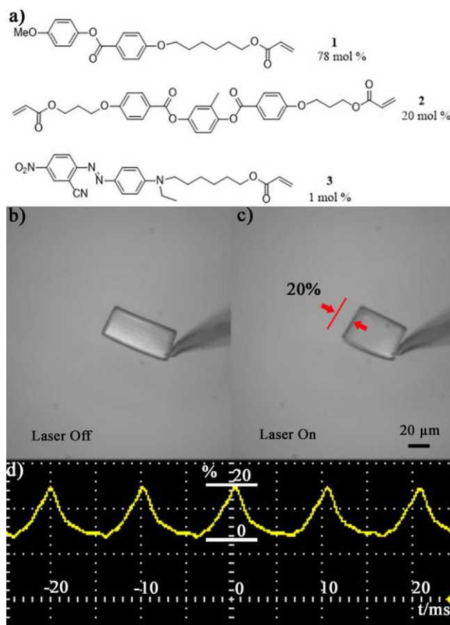
Figure 1. Liquid crystalline monomers composition and actuating response of a Liquid-Crystalline Elastomer (LCE) micro-structure.
