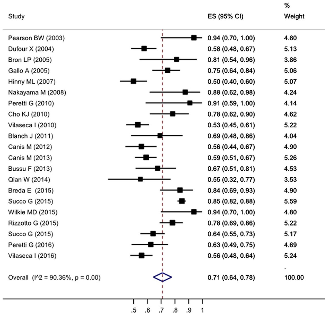
Fig. 2 Forest plot of overall survival (OS) for all patients, with pooled estimate and confidence intervals calculated using the DerSimonian Laird (random effects) model
