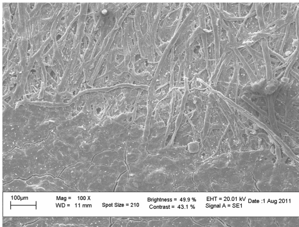
Fig. 4. SEM image of an untreated paper specimen showing the boundary line between the glue coating (bottom) and the cellulose fibres (top) [100 \times ; scale-bar 100 \mu m].
