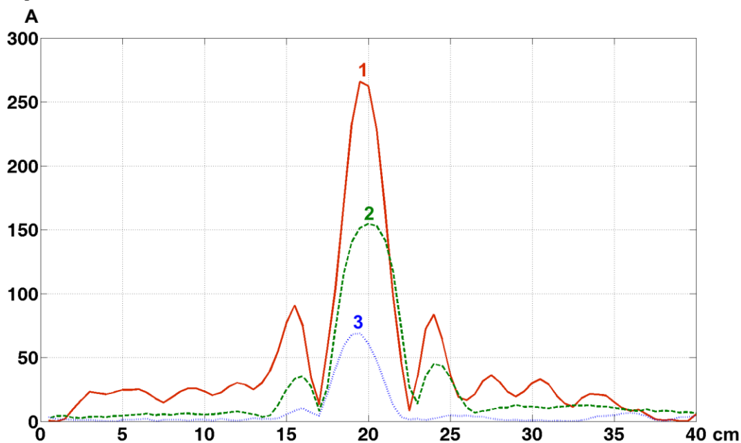
Fig. 12. Influence of attenuation of electromagnetic wave in medium on character of recorded holograms: 1. The wire is under four dry plaster sheets 2. The wire between two dry bricks 3. The wire between two wet bricks.
