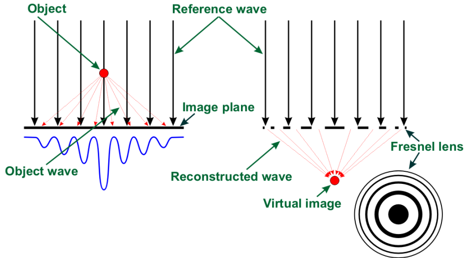
Fig. 1. The principle of simplest optical hologram proposed by D. Gabor.
