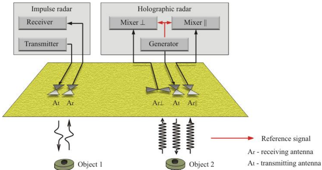
Fig. 3. Comparison of impulse and holographic radars schemes
