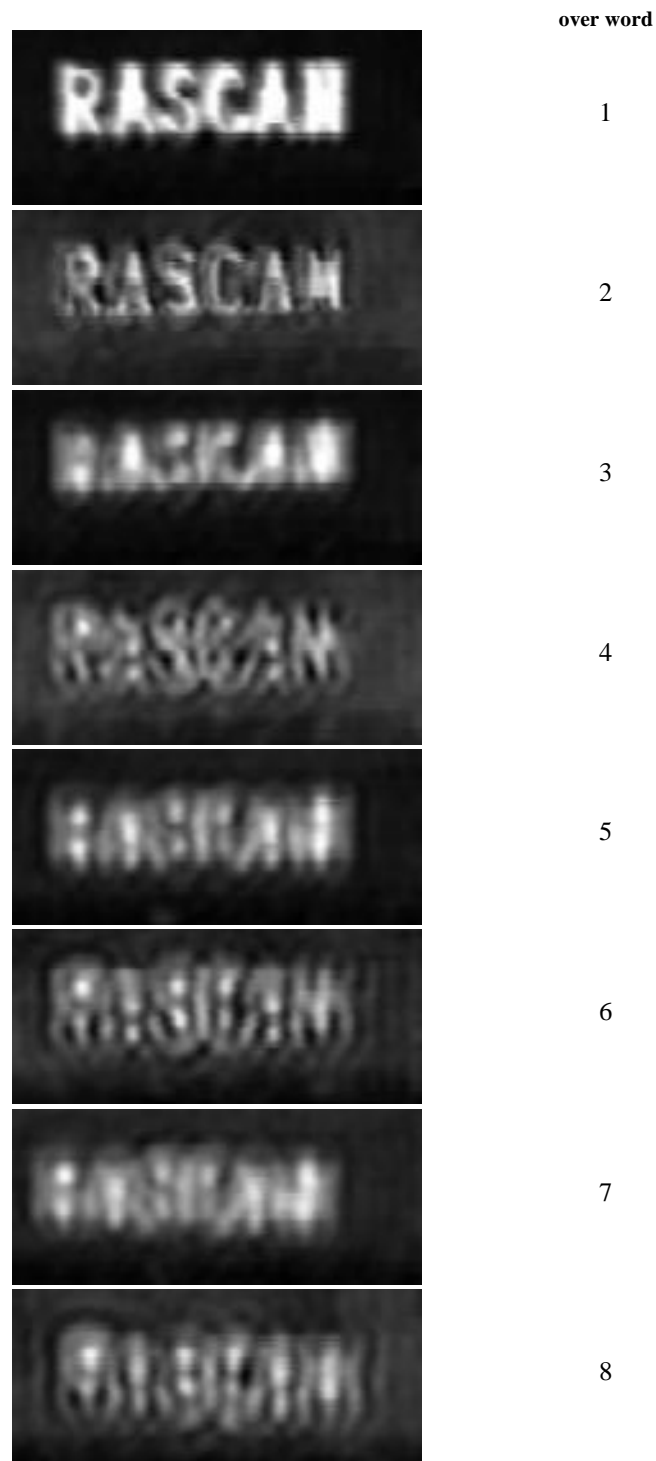
Fig. 8. RASCAN holograms recorded through the stack of plaster sheets. Depth is 1.2 cm per sheet.
