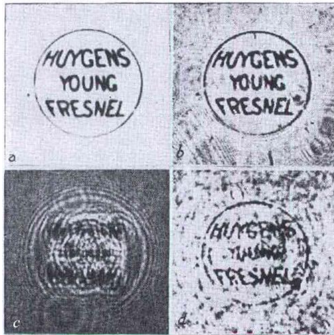
Fig. 9. Gabor's hologram [4]: a) Original micrograph b) Micrograph, directly photographed through the same optical system which is used for the reconstruction d) c) Interference diagram d) Reconstruction of the original; the letters have again become legible.
