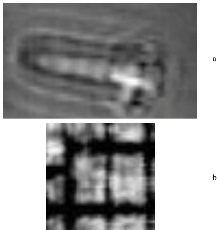
Fig. 11. Influence of medium attenuation level on character of recording holograms: a) Radar hologram of 50mm rocket in dry sand [5] b) Hologram of a part of ferroconcrete wall [16].
