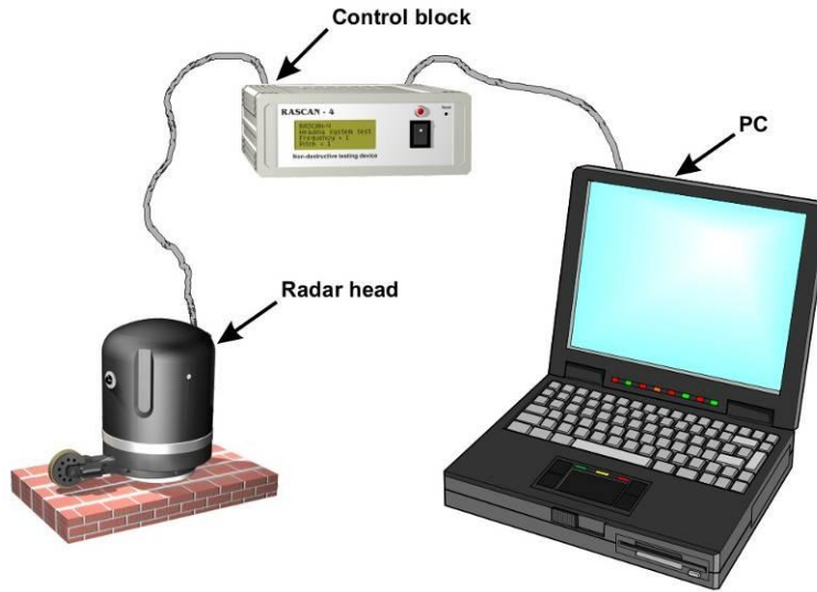
Fig 4. Connection scheme of the RASCAN-4 radar parts with computer.
