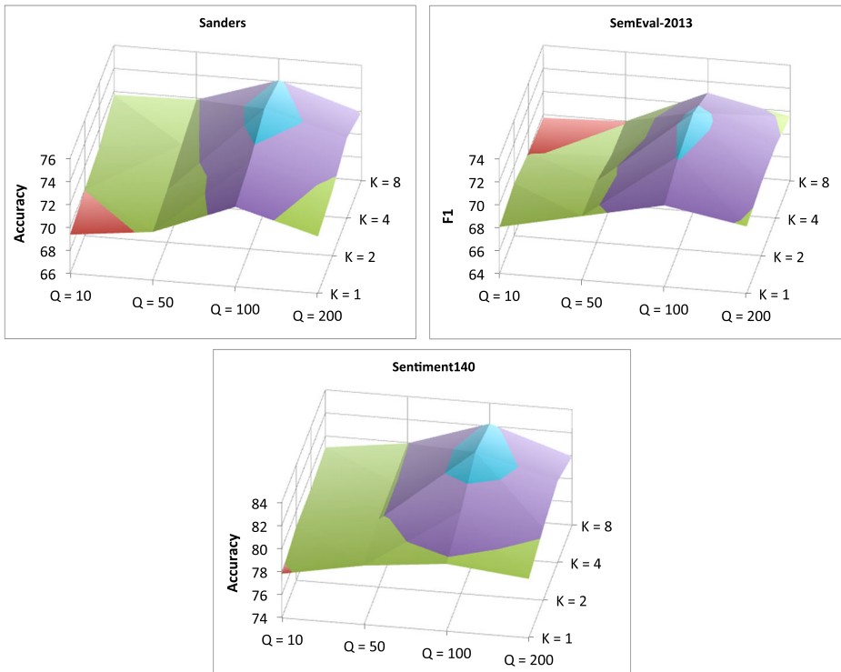
Fig. 5 Performance of the proposed method when varying K and Q parameters on Sanders, SemEval-2013 and Sentiment140 datasets
