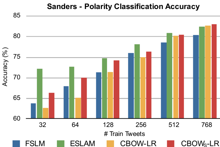
Fig. 4 Comparison between our method with FSLM and ESLAM [28] on Sanders dataset, while varying the number of training tweets
