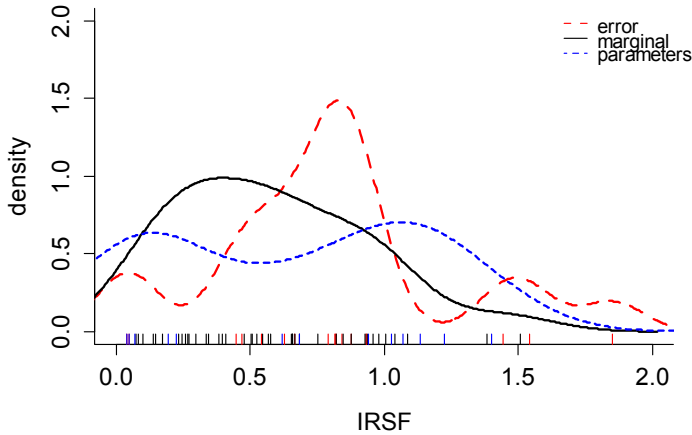
Figure 1. Density estimates of IRSF.
