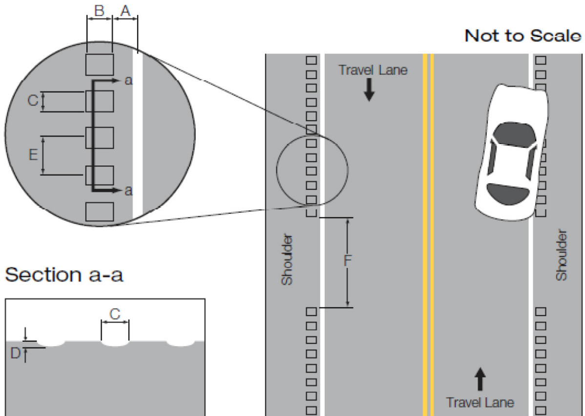
Figure 21: Design parameters for shoulder rumble strips [21]
