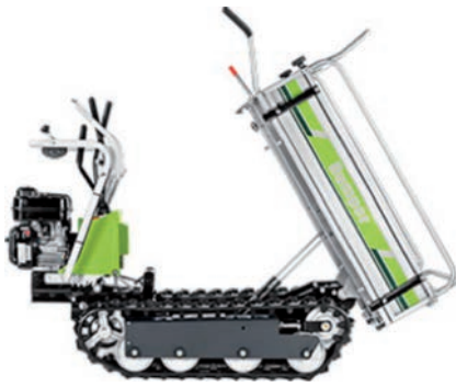
Figure 1. Grillo – mini crawler dumper- 406. The compact size (161×71×110 mm) permit to work in narrow space. The driving position is on the ground, it is provided with the automatic parking brake. Manual tipping.
