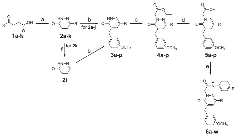
Scheme 1. Synthesis of pyridazin-3(2H)-one derivatives 6a–w . Reagents and conditions: a) NH_2NH_2 (1 equiv), EtOH, 1–3 h, 60 °C; b) 3 or 4-methoxybenzaldehyde (1 equiv), KOH 5% (w/v) in anhydrous EtOH, 1–3 h, reflux; c) ethyl bromoacetate (1.5 equiv), K_2CO_3 (2 equiv), anhydrous CH_3CN , 1–3 h, reflux; d) NaOH 6N, 1–2 h, 60–80 °C; e) ethyl chloroformate (1.1 equiv), Et_3N (3.5 equiv), substituted aniline (2 equiv), anhydrous THF, 12 h, –5 °C/rt; (f) 0.5 h, 160 °C.
