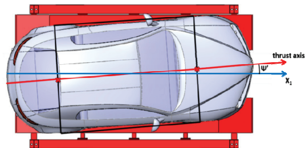
Figure 10. Run-out effect due to misalignment of the vehicle
