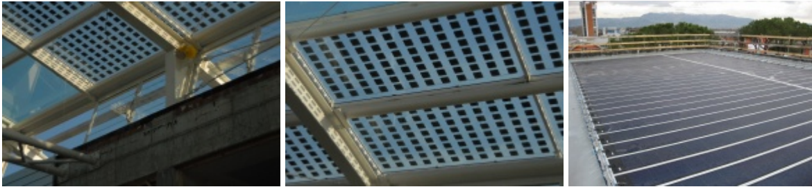
Figure 2. (a,b,) Details of the photovoltaic atrium integrated roof from inside. (c) Detailed of the thin film integration on the roof
