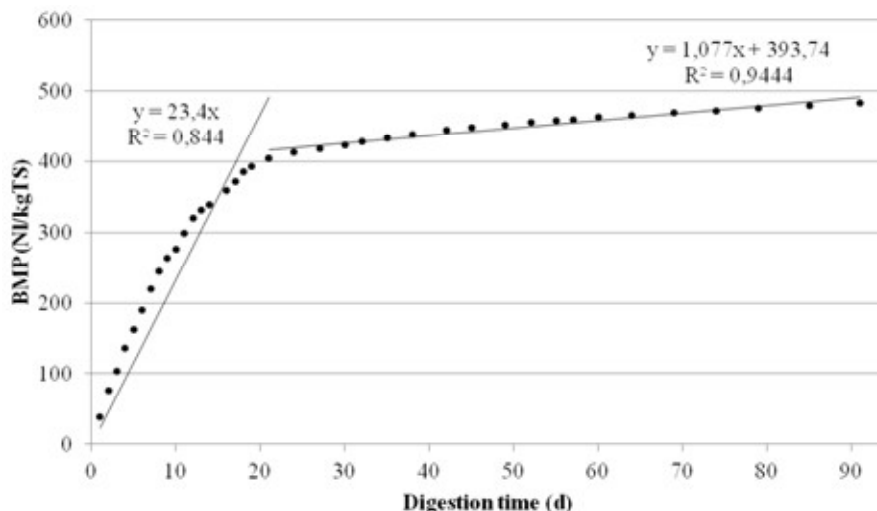
Fig. 10: MFW BMP schematization
