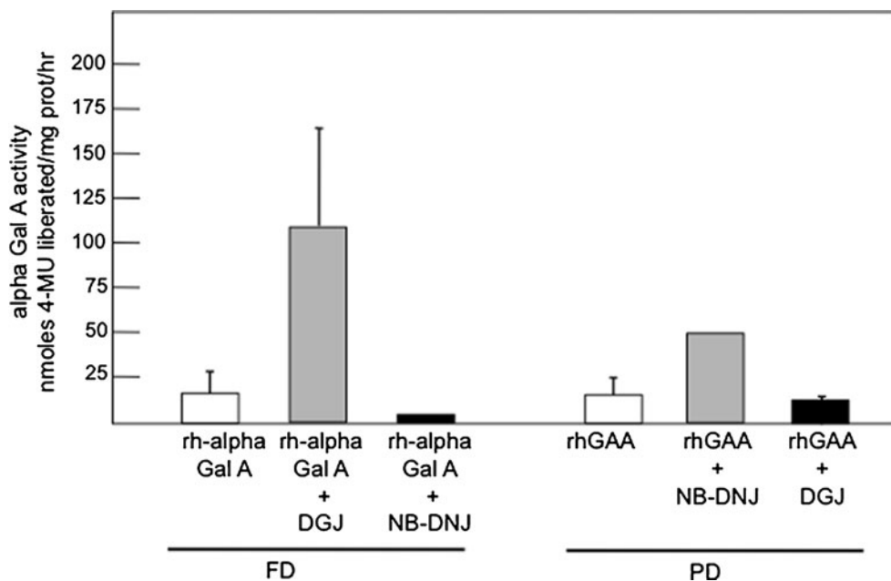
Fig. 3 Effect of different chaperones on recombinant enzymes. FD cell lines incubated with rh-alpha-Gal A in the presence of NB-DNJ, a known chaperone for GAA, showed no enhancement of GLA activity. Similarly, no effect was seen on GAA activity in PD fibroblasts treated with GAA in the presence of DGJ. GAA activity was assayed as described in Porto et al. (2009)
