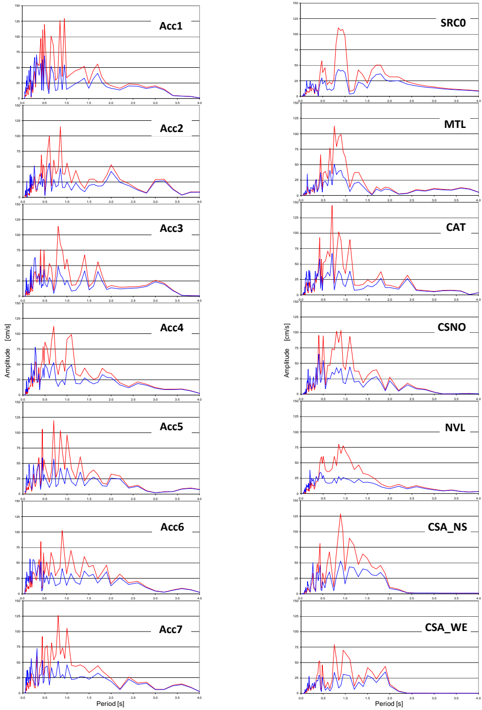
Figure 4. Fourier spectra of the acceleration time histories obtained by means of local seismic response analyses (red lines) adopted artificial (left column) and recorded (right column) signals (blue lines) (after Pergalani e Compagnoni, 2008).
