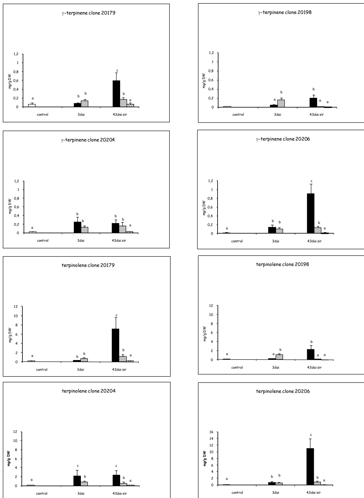
Figure 10: Enantiomeric profiles (mg moterpenes/ g tissue) of terpenes in Sitka spruce clones. Terpenes increased in inoculated tissues. Letters indicate significant differences ( p < 0.05 )
