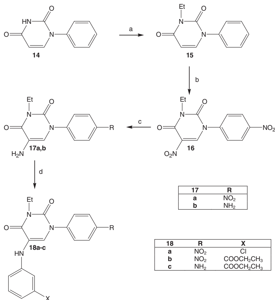
Fig. 3. Synthesis of 5-(substituted)anilino pyrimidine-2,4-diones 18a,b . Reagents and conditions: (a) EtBr, DMF, K 2 CO 3 , 90°C, 1 h; (b) KNO 3 , conc. H 2 SO 4 , rt, 8 h; (c) SnCl 2 , conc HCl, rt, 1 h; (d) ArB(OH) 2 , CH 2 Cl 2 , Ac 2 Cu, Et 3 N, rt, 24 h.
