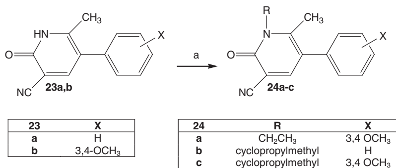
Fig. 5. Synthesis of 1-alkylpyrimidones 24a-c . Reagents and conditions: (a) RBr, DMF (or CH 3 CN), K 2 CO 3 , 90°C, 1h.
