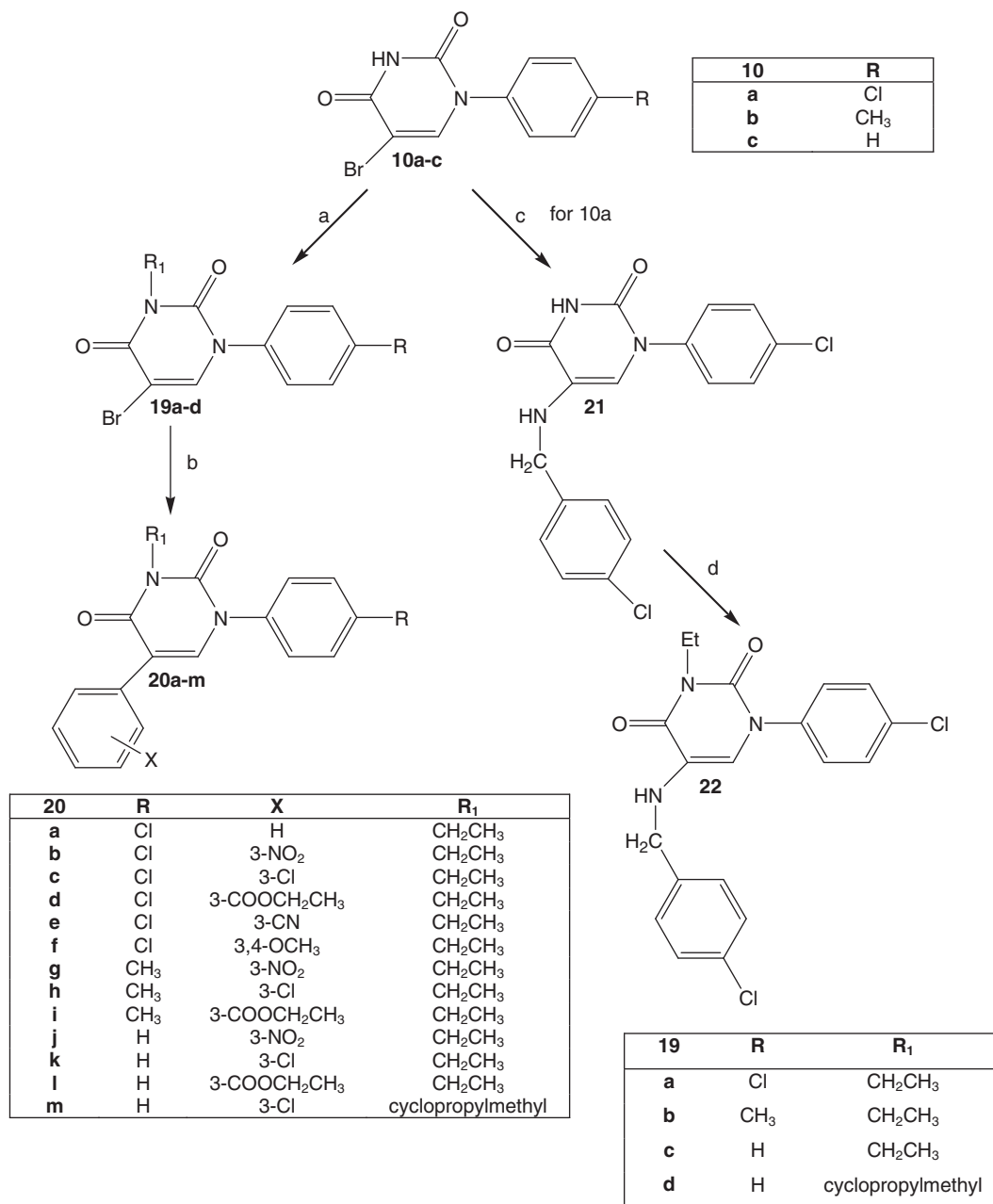
Fig. 4. Synthesis of 5-(substituted)phenyl pyrimidine-2,4-diones 20a-m and of compound 22 . Reagents and conditions: (a) R 1 Br, DMF, K 2 CO 3 , 90°C, 1 h; (b) X-C 6 H 5 -B(OH) 2 , Pd(PPh 3 ) 4 , 2M Na 2 CO 3 , toluene, 90°C, 16h; (c) 4-chlorobenzylamine, EtOH, 90°C, 9h; (d) EtBr, DMF, K 2 CO 3 , 90°C, 1h.
