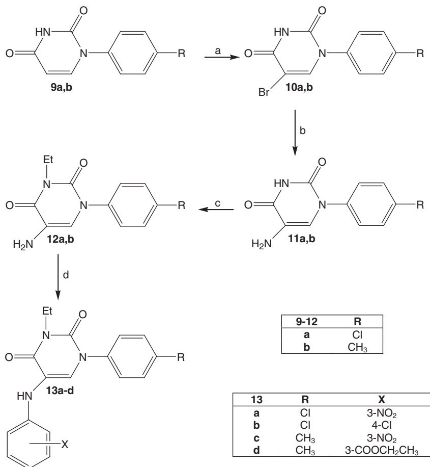
Fig. 2. Synthesis of 5-(substituted)anilino pyrimidine-2,4-diones 13a-d . Reagents and conditions: (a) Br 2 , AcOH 100%, rt, 3h; (b) NH 4 OH 33%, sealed tube, 120°C, 5 h; (c) EtBr, DMF, K 2 CO 3 , 90°C, 1h; (d) X-C 6 H 5 -B(OH) 2 , CH 2 Cl 2 , Ac 2 Cu, Et 3 N, rt, 24 h.
