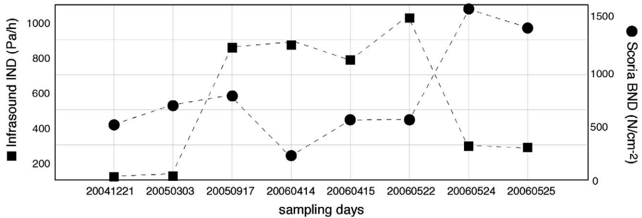
Fig. 5. The total number of bubbles (BND in \text{cm}^{-2} ) in each scoria is compared with the overall level of explosive degassing activity, represented by the total number of infrasonic amplitudes (IND) and calculated as the area below the IAD of Fig. 2a. Small BND reflects a large contribution of big bubbles to the scoria vesiculation and, in general, correlates with a period of high infrasonic activity (large IND) and with periods of high explosive degassing regime. This correlation is good enough (correlation coefficient 0.61) to support an explosive degassing model controlled by a bubble accumulation process.
