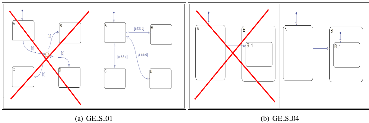
Figure 1: Two examples of the GETS modeling rules
