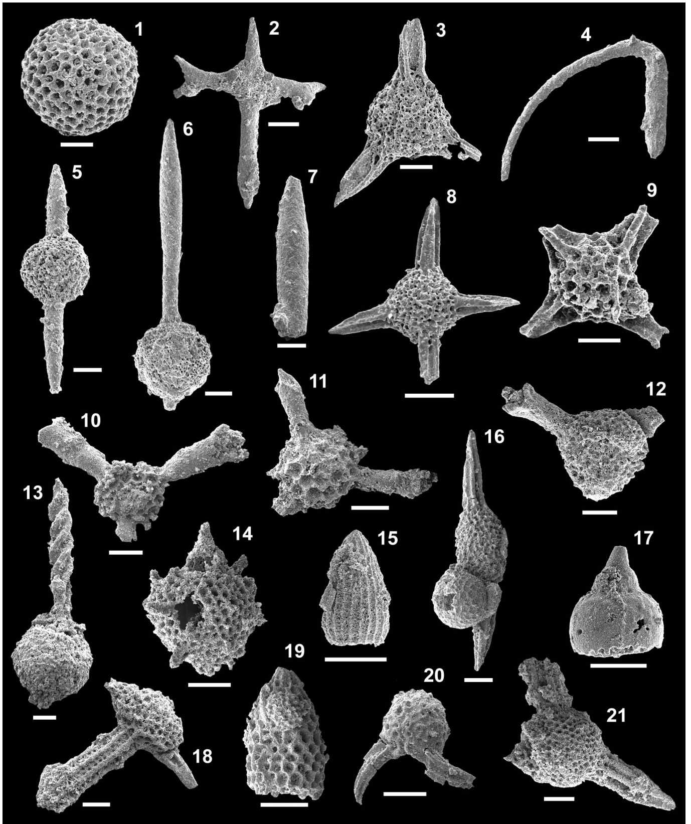
Plate 1 Middle Triassic . 1 Archaeocenosphaera sp. cf. A. clathrata (Parona), VR16; 2 Baumgartneria bifurcata Dumitrica, VR3; 3 Eptingium manfredi Dumitrica, VR16; 4 Oertlispongia inaequispinosa Dumitrica, Kozur and Mostler, VR3; 5 Pararchaeospongoprunum sp. cf. P. hermi Lahm, VR16; 6 Paroertlispongia multispinosa Kozur and Mostler, VR16; 7 Paroertlispongia multispinosa Kozur and Mostler, VR5; 8 Plafkerium sp., VR16 9 Tiborella florida (Nakaseko and Nishimura), VR16.
