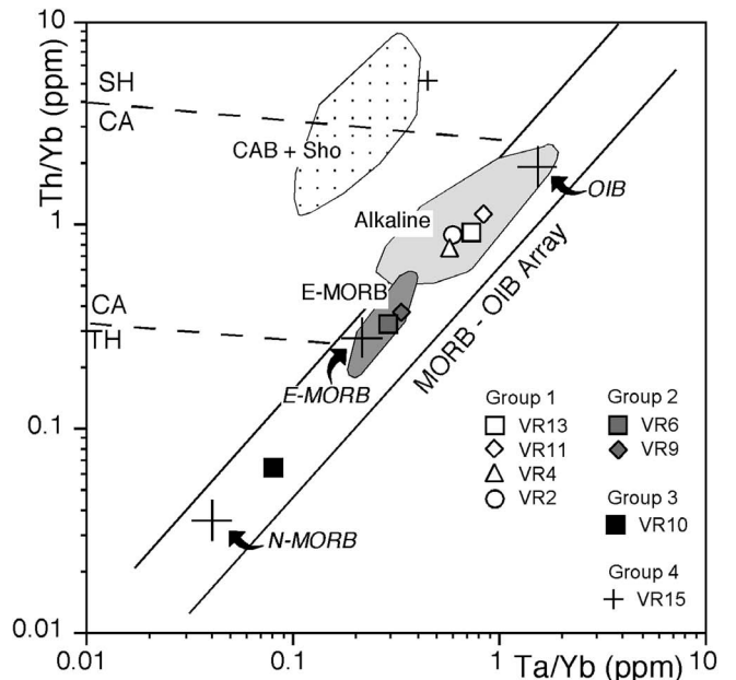
Fig. 5 - Th/Yb vs. Ta/Yb diagram for volcanic rocks from the mélangé. Large crosses indicate the compositions of Modern ocean-island basalt (OIB), enriched-type mid-ocean ridge basalt (E-MORB), and normal-type mid-ocean ridge basalt (N-MORB), according to Sun and McDonough (1989). Variations of elemental ratios of Triassic calc-alkaline basalts (dotted field), Triassic alkaline basalts (light gray field), and E-MORBs (dark gray field) from various localities of the Hellenides are reported for comparison (data from Pe-Piper and Piper, 2002; Saccani and Photiadis, 2005, and references therein).
