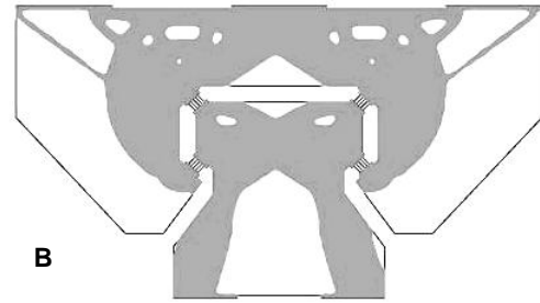
Figure 12: Topologically optimized density distribution of a linear guidance corresponding to the load cases 1 (above, A) and 2 (below, B) of figure 11.
