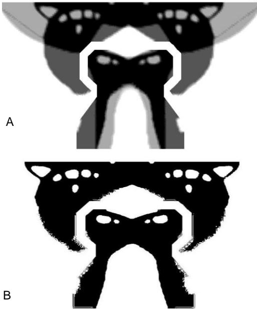
Figure 14: Above (A): hybrid solution obtained through the application of formula (1) to topologies “A” and “B” of figure 12. Below (B): resulting topology after applying a threshold equal to 0.85 to the density distribution in order to have a total mass of 16.5 kg/m.
