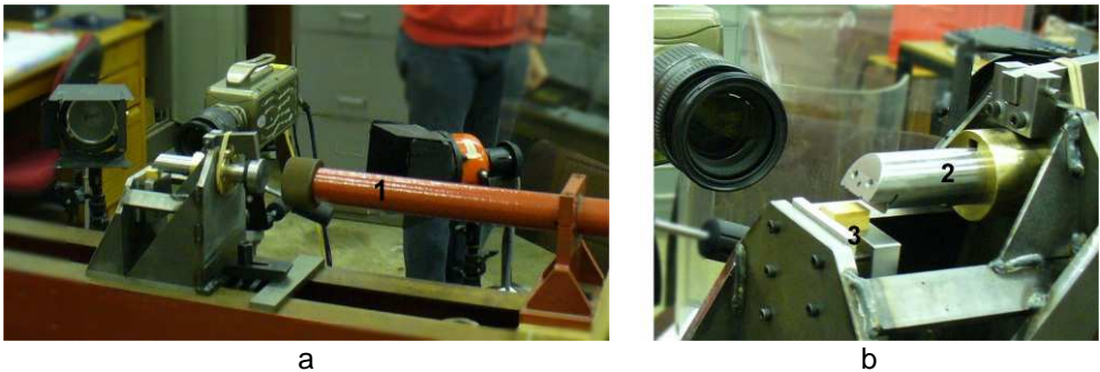
Figure 2. The adapted Hopkinson's Bars system used in the high speed tests.
