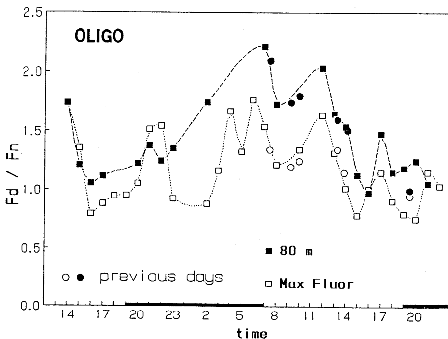
fig. 3 - Time series of variation for the F_d/F_n ratio (fluorescence with and without DCMU) at 80 m and at the fluorescence maximum of st. 02. Some measurements are added, made at st. 02 at the same depths, during the previous days.
