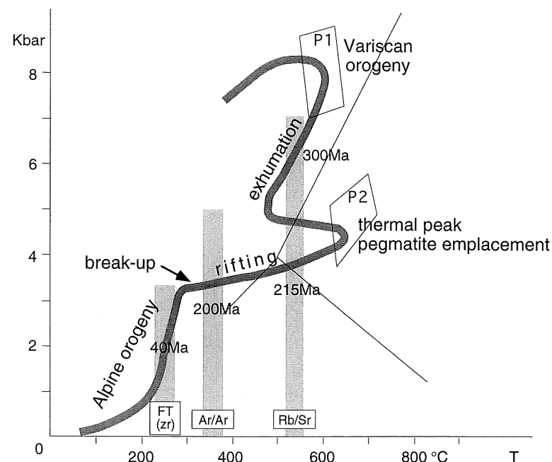
Fig. 11. P-T-t path for the tectonometamorphic evolution of the Piona crustal segment.
