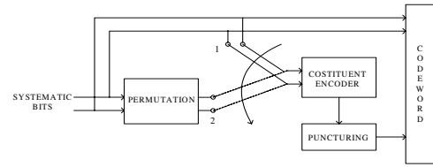
Fig. 3. Duo-binary Turbo Encoder
