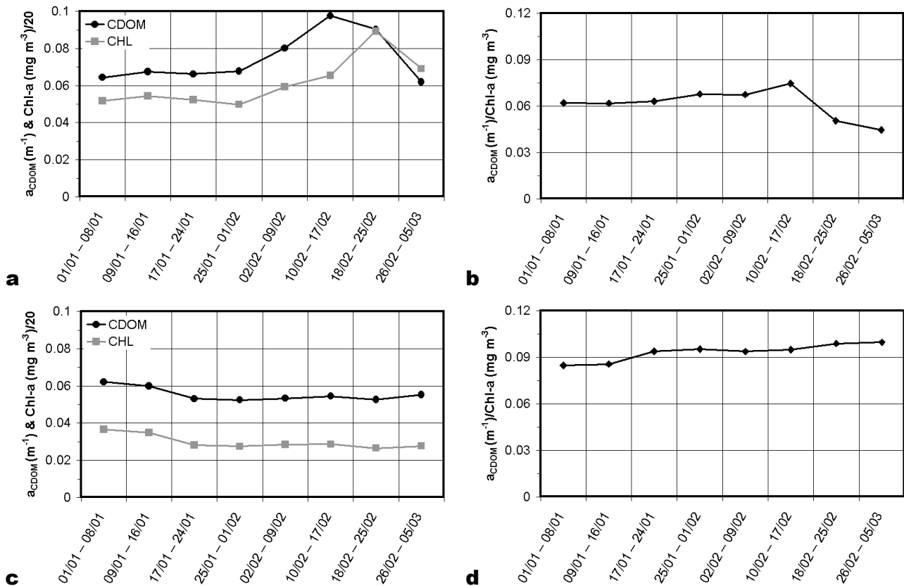
Figure 5: a_{\text{CDOM}} (black circles) and Chl-a (grey squares) averaged in Ross Sea Region (a) and their ratio (b) during the oceanographic campaign; a_{\text{CDOM}} (black circles) and Chl-a (grey squares) averaged in Ross Sea Sector (c) and their ratio (d) during the oceanographic campaign.
