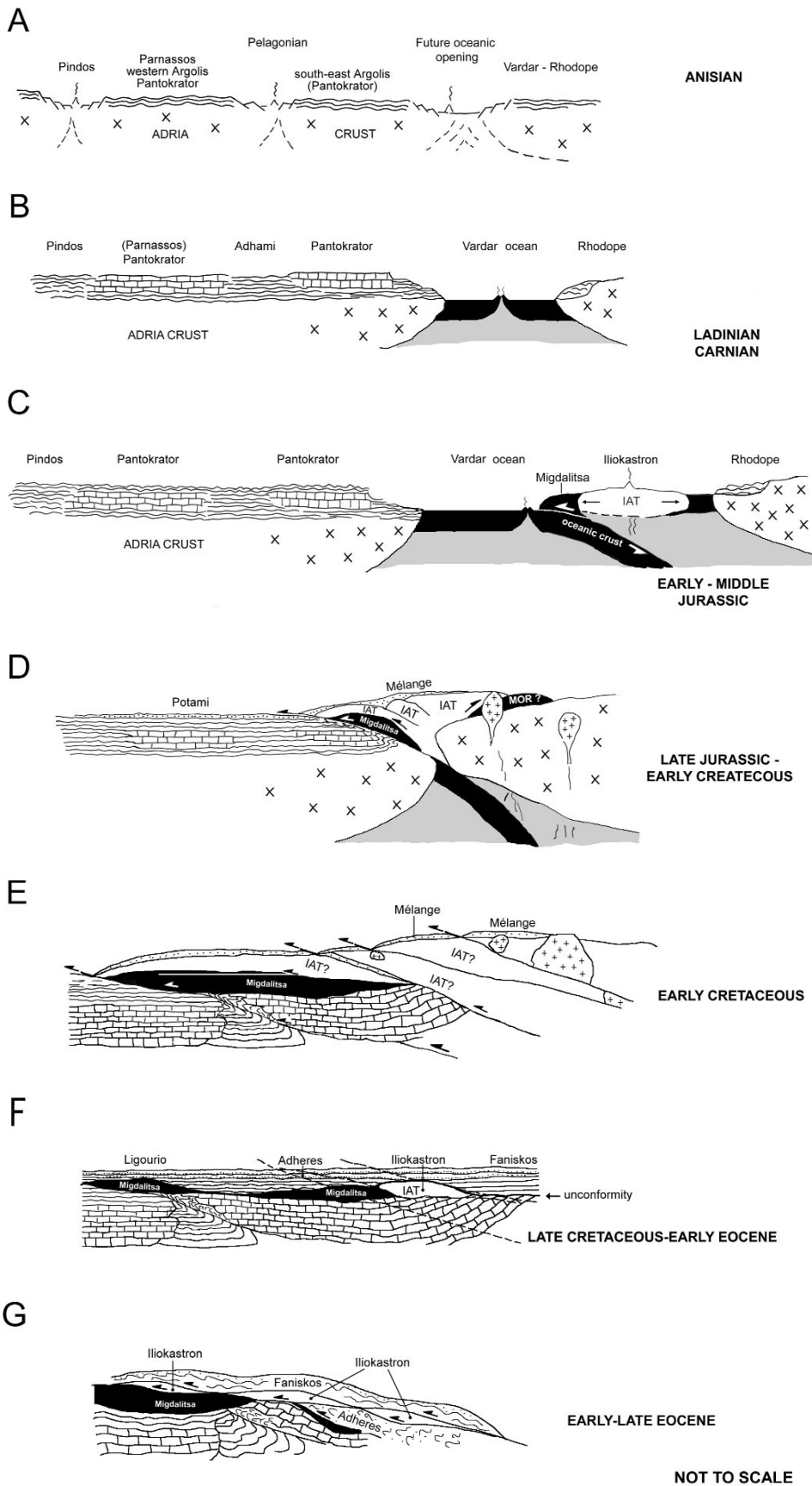
Fig. 5 - Scheme of the geodynamic evolution of the Vardar (Migdalitsa) Ocean and the Argolis continental margin from Triassic to Eocene.
