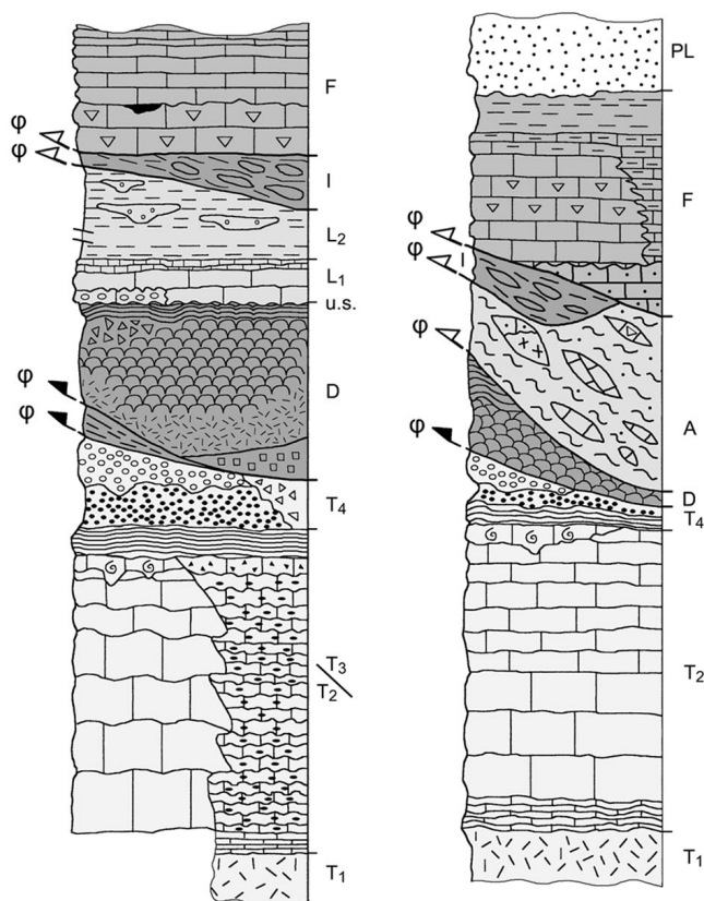
Fig. 4 - Tectono-stratigraphic logs of the Argolis Peninsula. A- northern Argolis; B- Southern Argolis. \phi - thrust contacts: For other symbols see Fig. 1.
