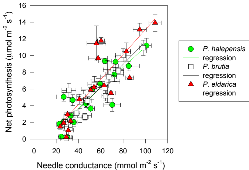
Fig. 5 - Linear relationship between net photosynthesis and needle conductance for P. halepensis , P. brutia and P. eldarica grown in an experimental plantation nearby Firenze (Italy). Data are the means \pm SE. Species are referred to by symbols in the legend. Parameters of regression equations ( P < 0.0001 ), y = a + bx , are the following: P. halepensis a = -1.19 , b = 0.12 , r^2 = 0.76 ; P. brutia a = -1.96 , b = 0.14 , r^2 = 0.84 ; P. eldarica a = -1.77 , b = 0.15 , r^2 = 0.73 .
