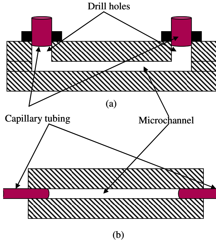
Figure 3.2-2: Schematic cross-section diagram showing microfluidic interconnections: (a) conventional interconnections where the capillary is inserted using drilled wholes on the cap/base wafer; (b) proposed interconnection scheme where the capillaries are inserted from the side opening which results from the premeditated design and wafer dicing
