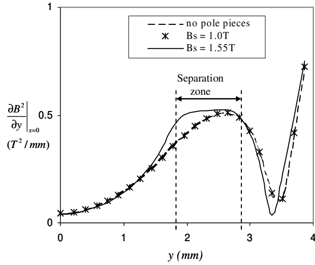
Figure 3.1-7: Graphs showing 2D simulation of \frac{\partial B^2}{\partial y} \Big|_{x=0} profile of the final design with different pole-piece materials.
