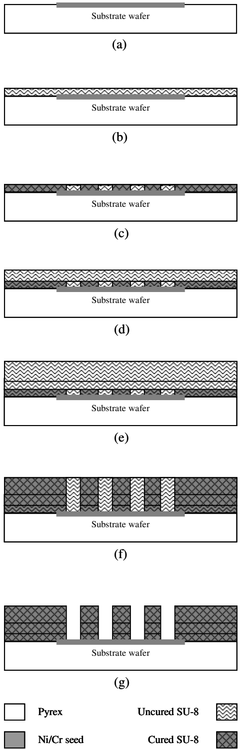
Figure 5.3-2: Schematic cross-section diagram showing different steps in fabricating the plating molds: (a) Start with substrate already patterned with the metal layer; (b) Spin-coat layer 1 (~10 μm) SU-8 and pre-bake; (c) Expose and PEB thin layer; (d) Spin-coat layer 2 (~20μm) SU-8 and pre-bake; (e) Spin-coat layer 3 (~100μm) SU-8 and pre-bake; (f) Expose layer 2 & 3 simultaneously; (g) Develop the three layers simultaneously
