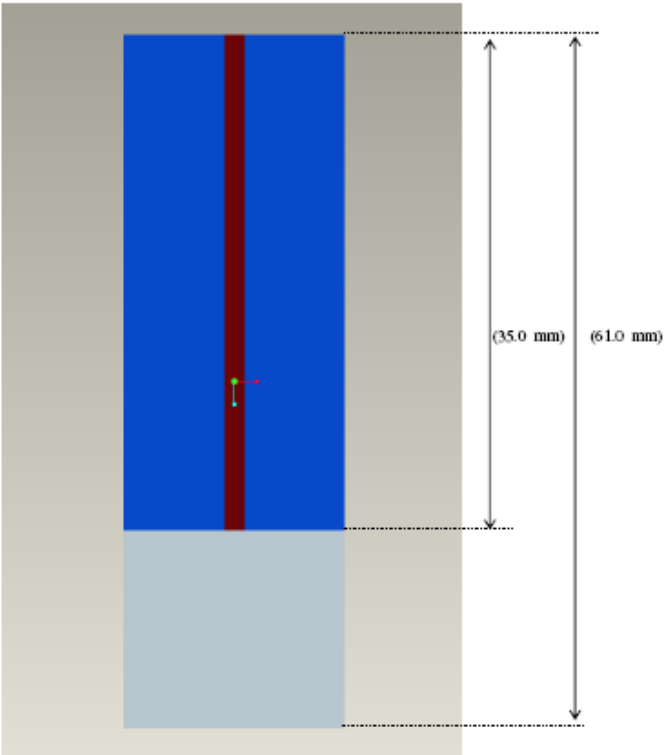
Figure C-4: Side view of the OGMS magnets with dimensions
