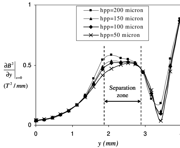
Figure 3.1-8: Graphs showing 2D simulation of \frac{\partial B^2}{\partial y} \Big|_{x=0} profile of the final design with different pole-piece heights ( h_{pp} ).
