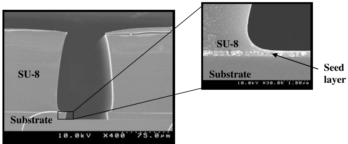
Figure 5.3-4: SEM micrograph showing cross-section of plating mold – the seed layer is exposed to allow flow of electrical charge
