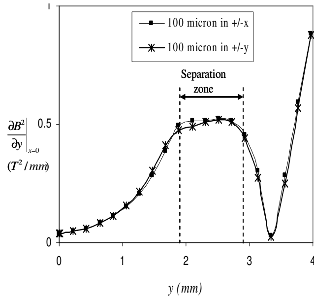
Figure 3.1-13: Graphs showing 2D simulation of \frac{\partial B^2}{\partial y} \Big|_{x=0} profile with different horizontal (mid-plane of the biochip is placed \pm 0.1 mm from the mid-plane of the magnetic circuit) and vertical displacements ( d = 1.9 or 2.1 mm).
