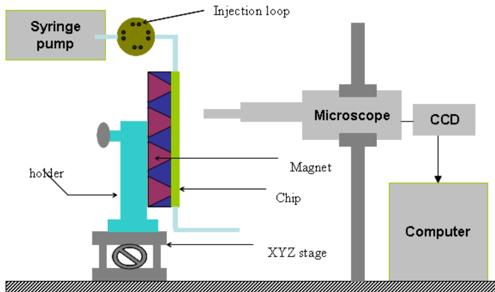
Figure 8.2-5: Schematic diagram showing the experimental setup for the multistage bio-ferrograph.
