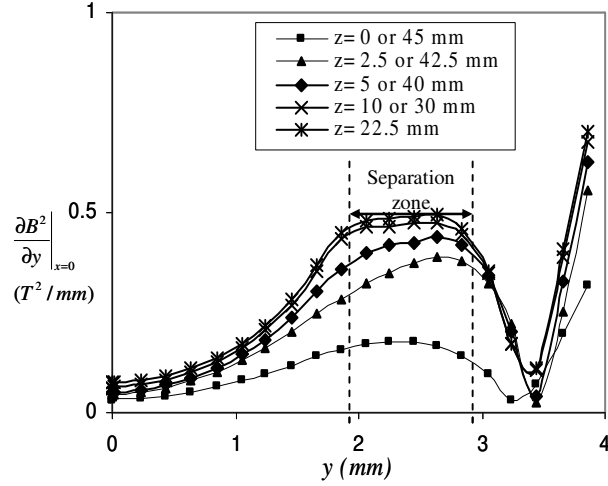
Figure 3.1-10: Graphs showing 3D simulation of \frac{\partial B^2}{\partial y}|_{x=0} profile of the final design.
