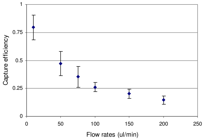
Figure 8.3-2: Graphs showing capture efficiencies of the multistage bio-ferrograph at different flow rates for a magnetic particle sample concentration of 1 \times 10^4 particles/ml.
