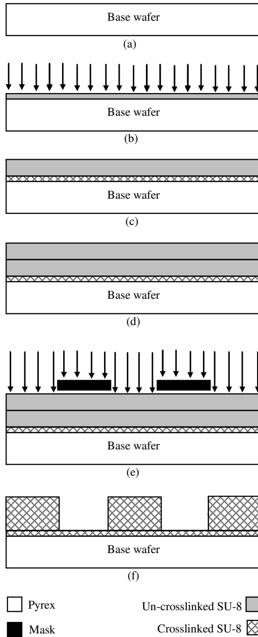
Figure 5.2-1: Schematic cross-section diagram showing the processing steps for the fabrication of open microchannels on Pyrex: (a) Piranha cleaned and dehydrated Pyrex wafer; (b) Apply \sim 10 \mu\text{m} SU-8 2010, soft bake, blanket expose and PEB; (c) Apply \sim 125 \mu\text{m} SU-8 2100 and soft bake; (d) Apply \sim 125 \mu\text{m} SU-8 2100 and soft bake; (e) Expose through mask to pattern the layers of SU-8 2100 simultaneously and PEB; (f) Develop SU-8 2100 layers
