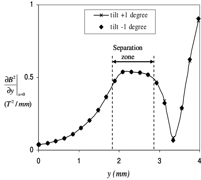
Figure 3.1-14: Graphs showing 2D simulation of \left. \frac{\partial B^2}{\partial y} \right|_{x=0} profile with different inclined positions
