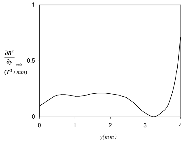
Figure 3.1-5: Graph showing 2D simulation of \left. \frac{\partial B^2}{\partial y} \right|_{x=0} profile of the initial discrete pole-pieces design.
