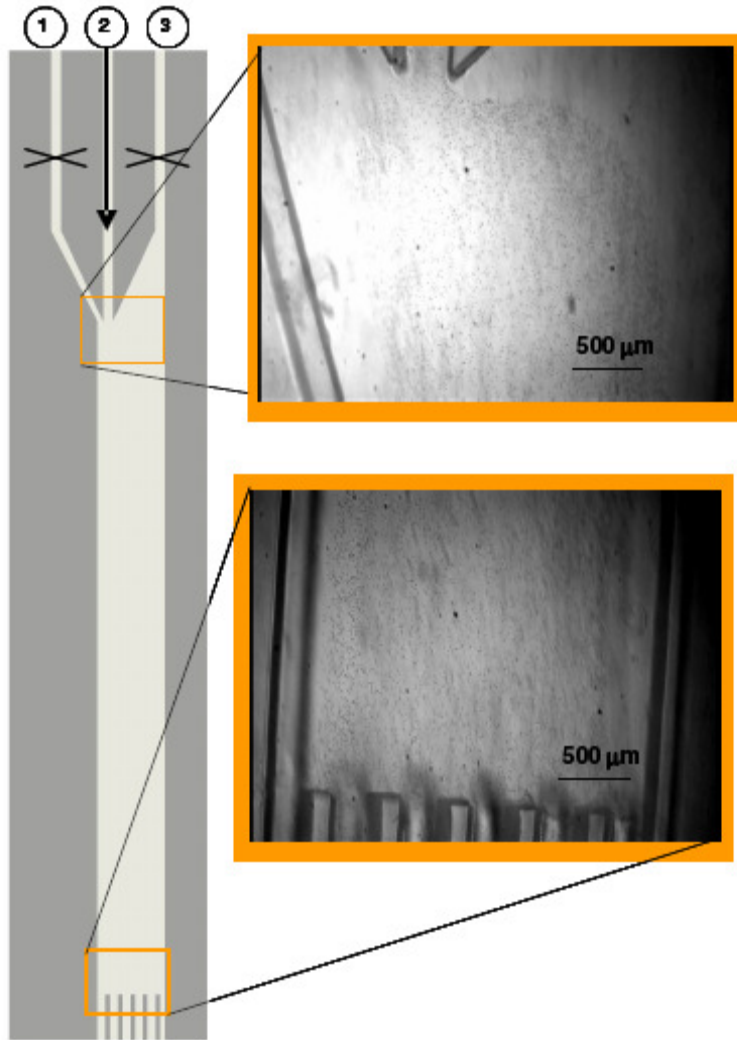
Figure 7.3-3: Optical microscope (5x) picture showing the flow of non magnetic particles inside the OGMS channel with no flows at inlet #1 and #3 - particles are spread throughout the cross-section of the channel and come out through all the outlets
