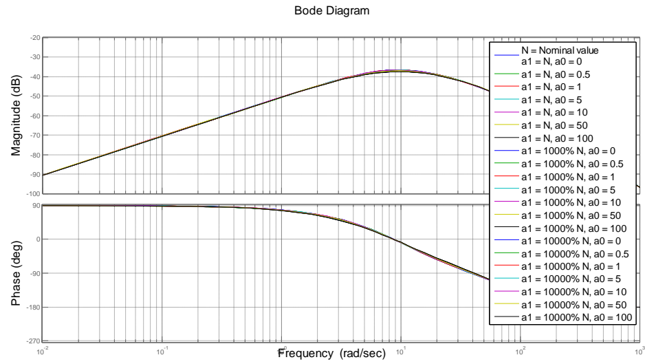
Figure 14: External disturbance rejection in the presences of the changes of a_0 and a_1
