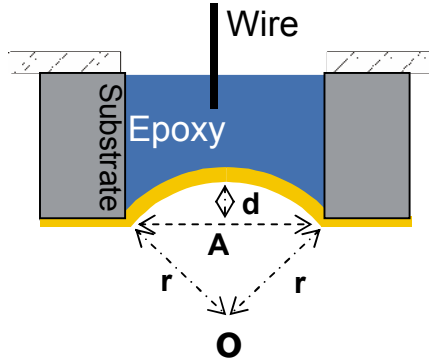
Figure 3.2-2: Cross-sectional view showing pertinent geometry of the focused transducer. The transducer has the ultrasound beam focused at a focal point ‘O’. Transducer focus can be controlled by changing the deflection ‘d’ which can be controlled by varying the air pressure during fabrication.
