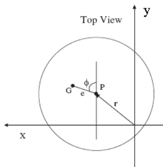
Figure 14: Rotation geometry (top view)
