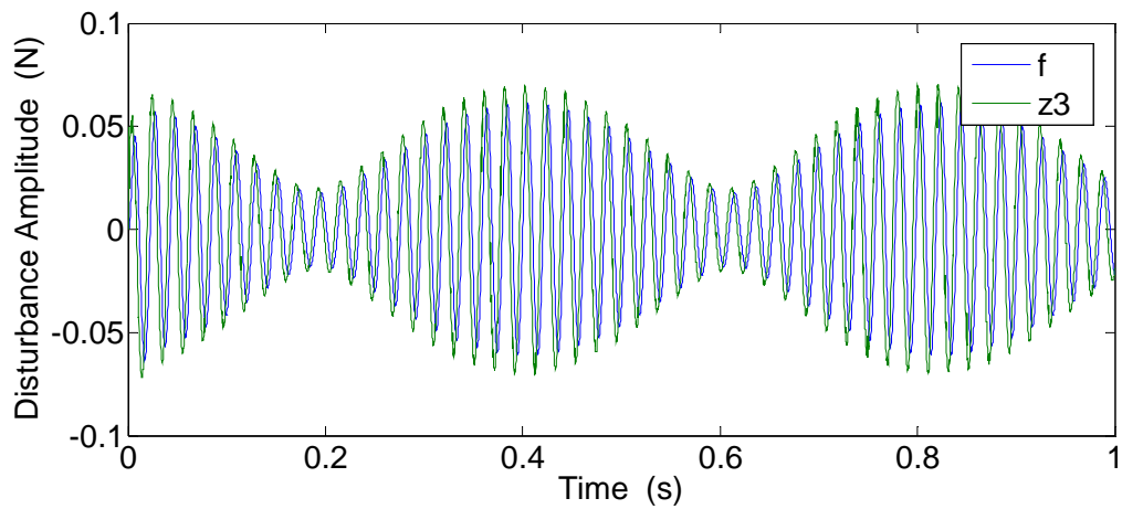
Figure 51: ESO tracking with lowered bandwidths ( \omega_o=1000 , \omega_c=200 )
