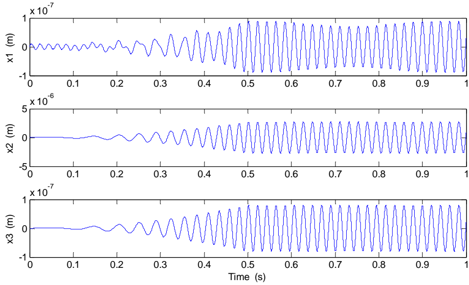
Figure 41: PID Control (displacement)
