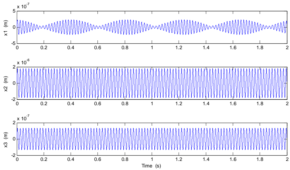
Figure 36: Three-Bearing PID Control (displacement)
