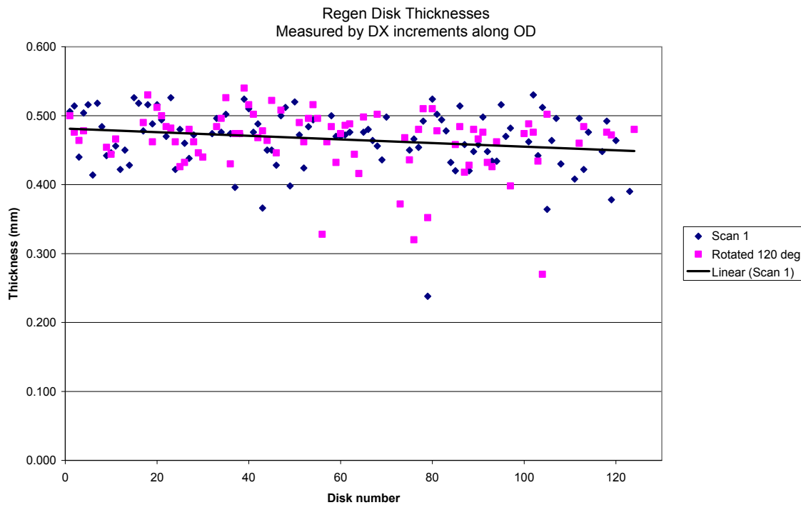
Figure 21.—Disk thickness measurements.
