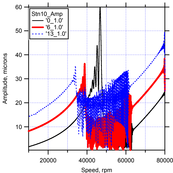
Figure 11: Deceleration data for 1 sec ramp time.
