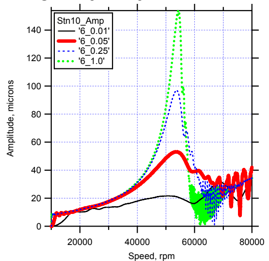
Figure 5: Speed ramp data for 6 \mu\text{m} IRC.
