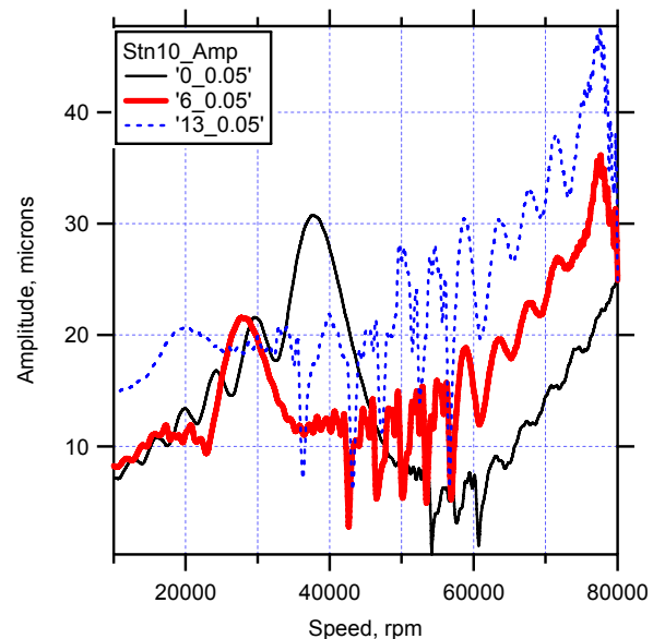
Figure 12: Deceleration data for 0.05 sec ramp time.
