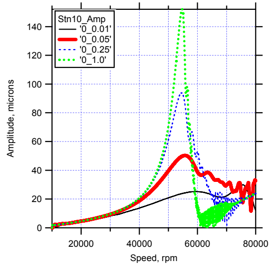
Figure 4: Speed ramp data with zero IRC.
