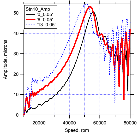
Figure 13: Acceleration data for horizontal rotor; ramp time, 0.05 sec.
