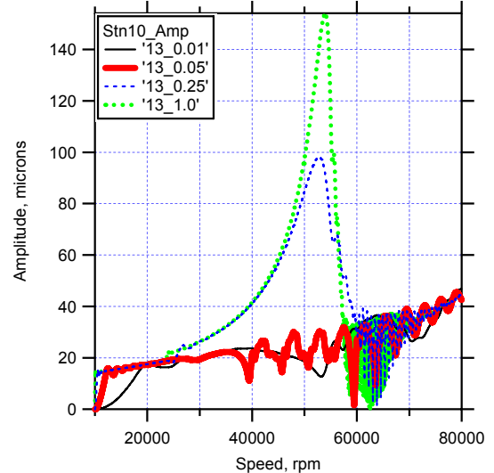
Figure 6: Speed ramp data for 13 \mu\text{m} IRC.
