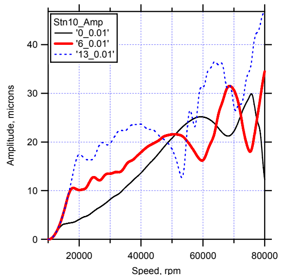
Figure 10: Acceleration data for 0.01 sec speed ramp.
