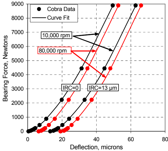
Figure 3: Load vs deflection for ball bearing.
