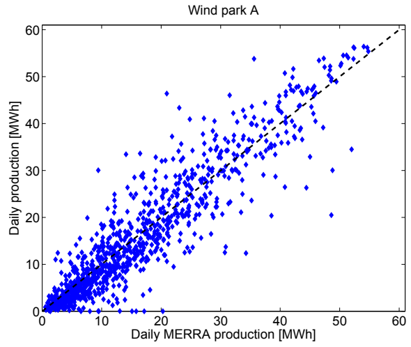
Figure 8: Daily MERRA production vs. true daily production
