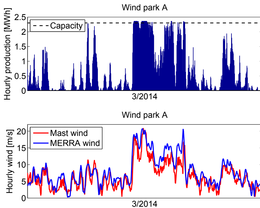
Figure 1: Hourly production and hourly average wind speed (mast and MERRA) for an exemplary month of wind park A
