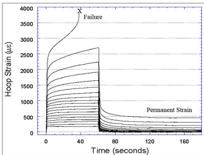
Figure 1. Multiphase loading illustrating creep, creep rate, failure and permanent strain.
