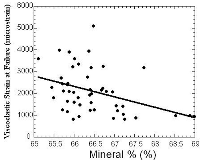
Figure 2. Variation in viscoelastic failure strain with mineral percentage.
