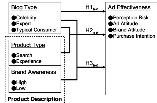
Figure 1 Research Framework
