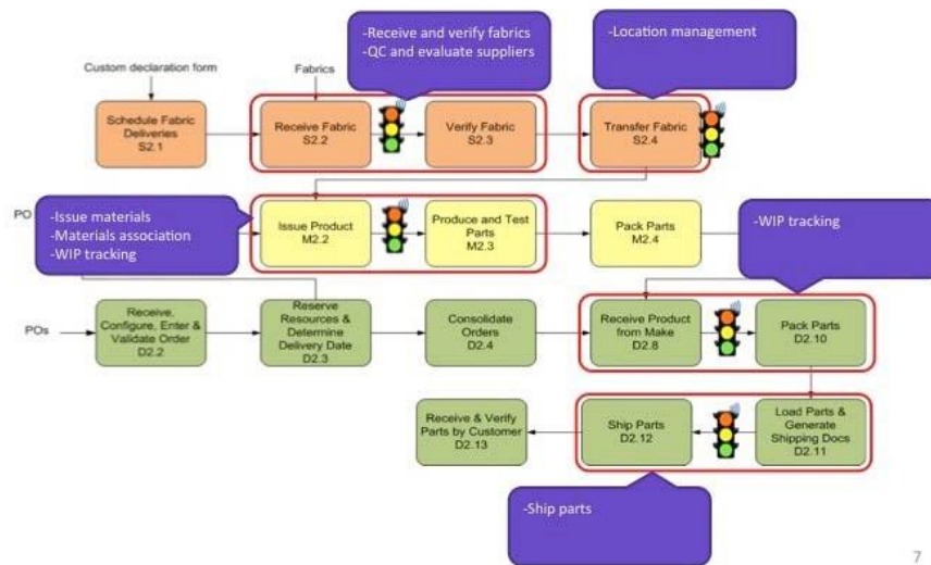
Figure 1. Enabling Visibility with RFID of a Garment Supply Chain
