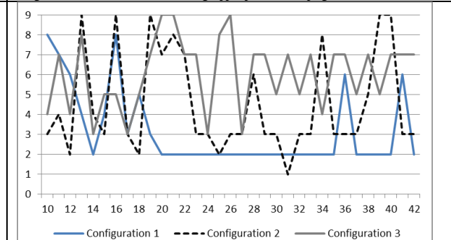
Figure 2d: Policy changes across configurations
