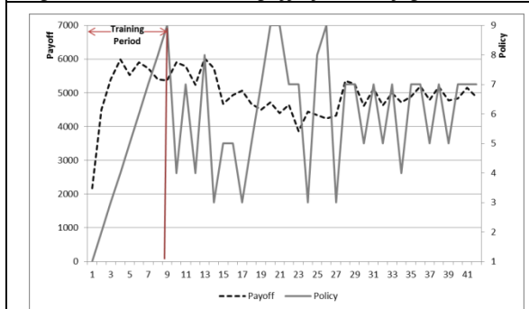
Figure 2c: Policies Payoffs for Configuration 3
