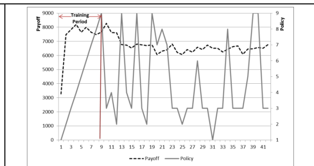
Figure 2b: Policies-Payoffs for Configuration 2
