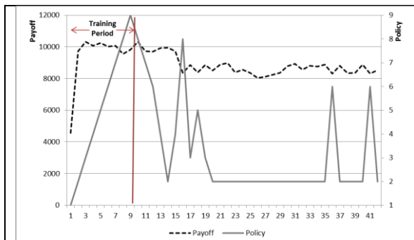
Figure 2a: Policies-Payoffs for Configuration 1
