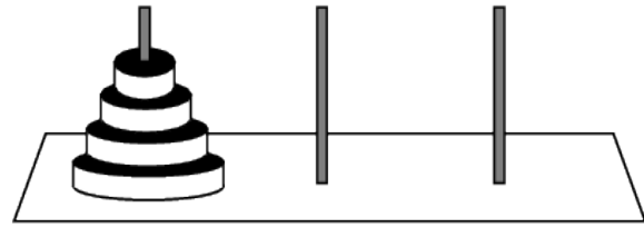
Figure 2. The Towers of Hanoi with 4 rings
