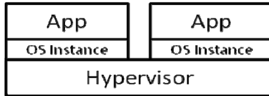
Figure 7. Application Virtualization
